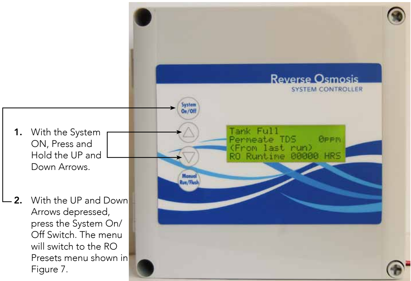
Figure 6. Controller Programming. Accessing the hidden menus.
