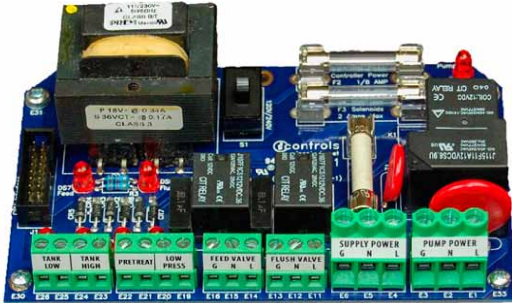
Figure 4. Controller Detail: Terminal Board, TB-1 (See Fig. 1 for schematic)
