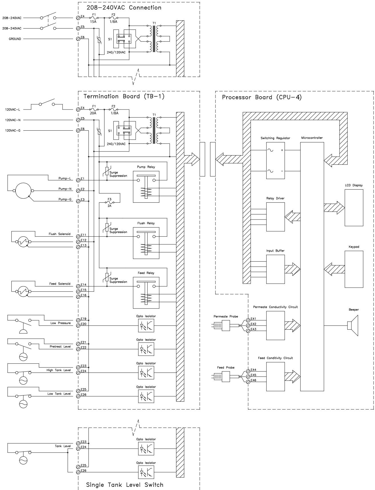
Figure 1. Simplified Schematic
